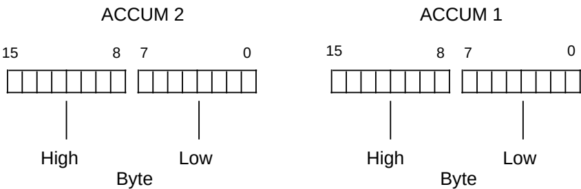
Figure 8-1. Accumulator Structure
