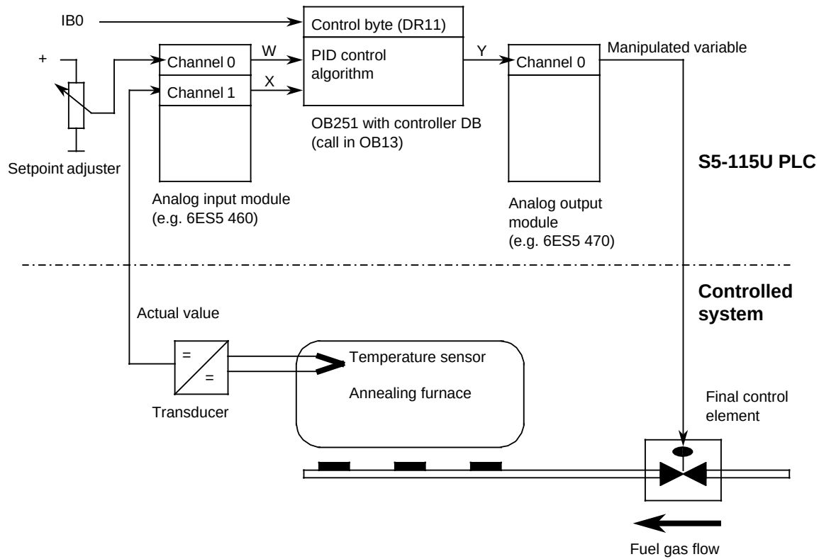
Figure 11-5. Process Schematic
