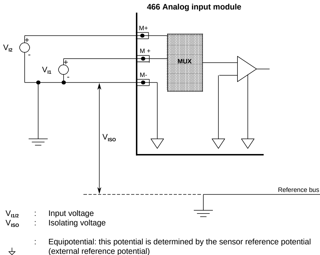
Figure 10-18. Connecting Transducers to the 466 Analog Input Module (Common-Reference Measurement)
