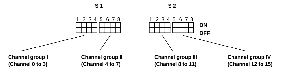
Figure 10-22. Assignment of Switches S 1/S 2 to Channel Group
